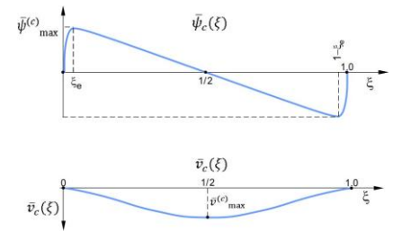
Fig. 12. Graphs of the dimensionless shear effect function (55) and the relative deflection (57) of the clamped beam
