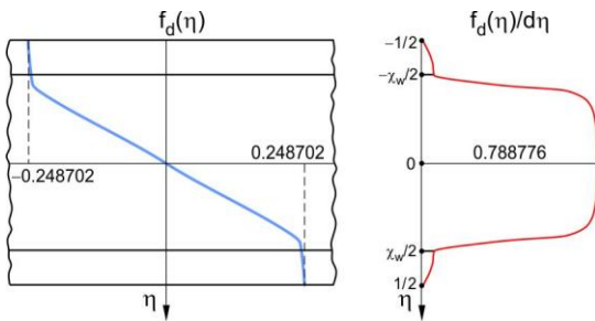
Fig. 14. Graphs of deformation functions f_d(\eta) and its derivatives df_d/d\eta of this beam
